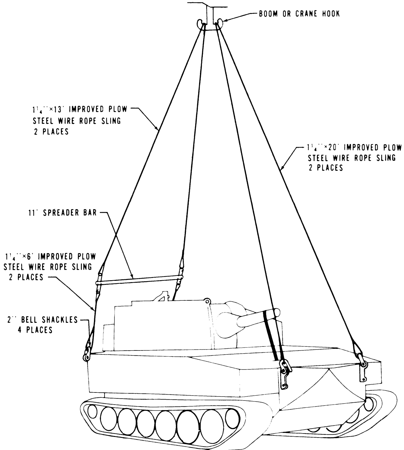
Figure 6-1. Lifting diagram for M108 using four-legged bridge sling and one spreader bar.
