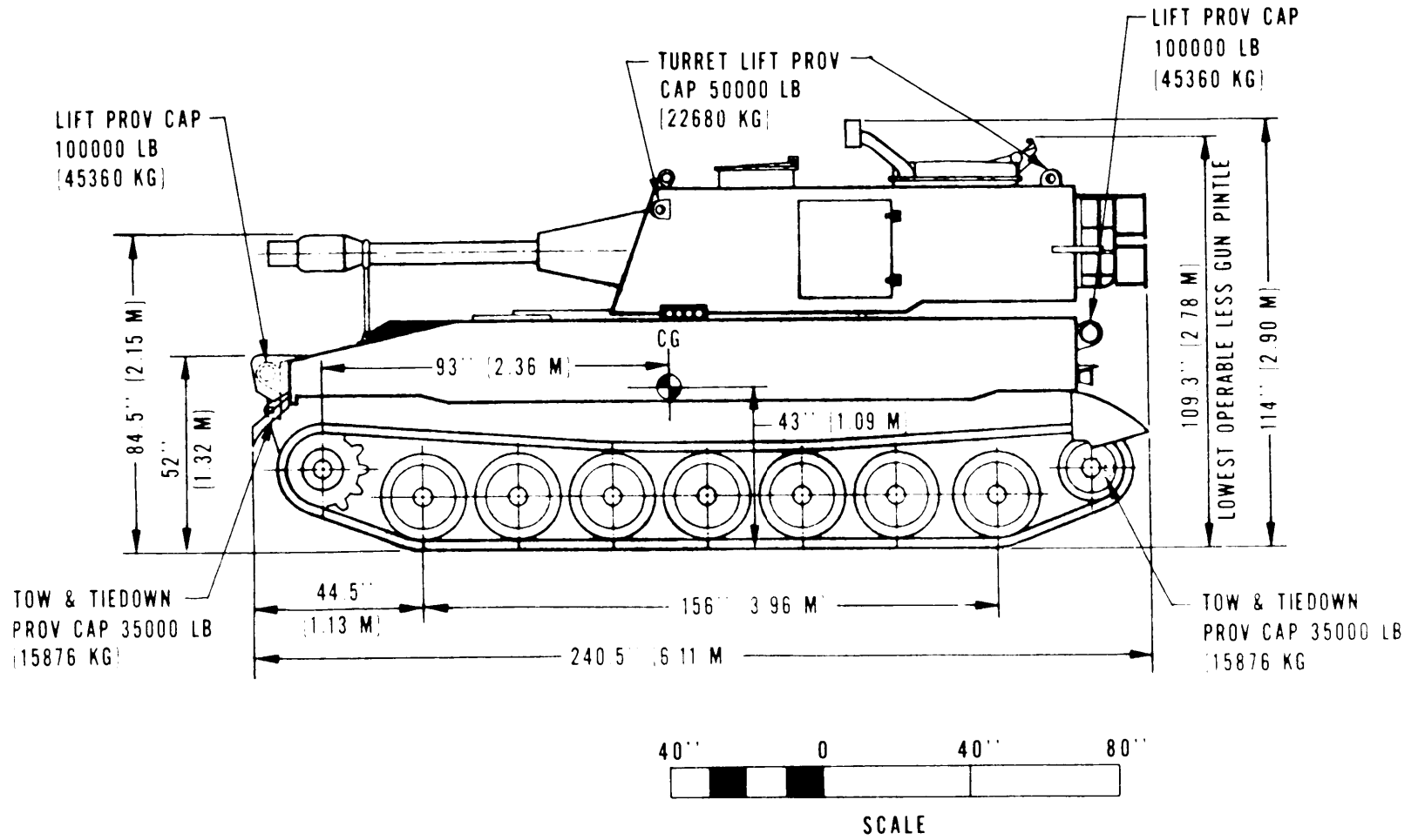
Figure 2-4. Side elevation, M108.
