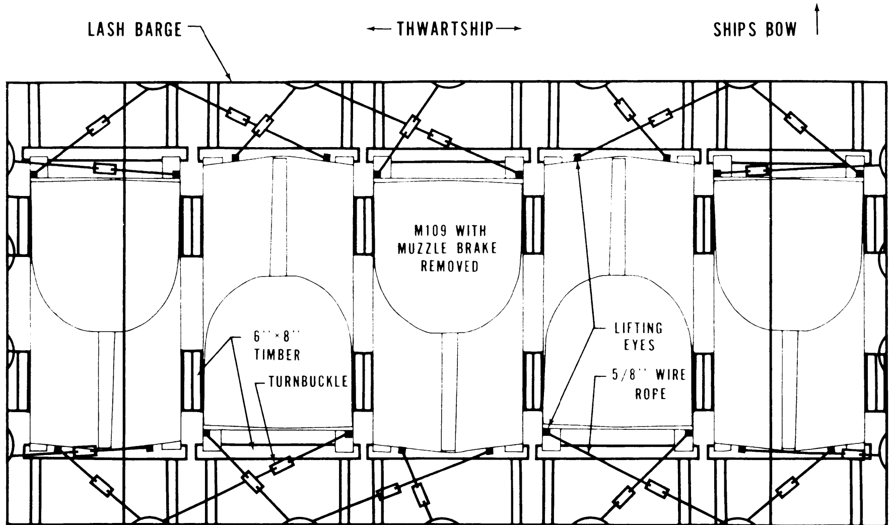
Figure 6-4. Loading of five howitzers, M109, on LASH barge, using wire rope, cable clamps, and turnbuckles, with blocking between howitzers and howitzers to hull.
