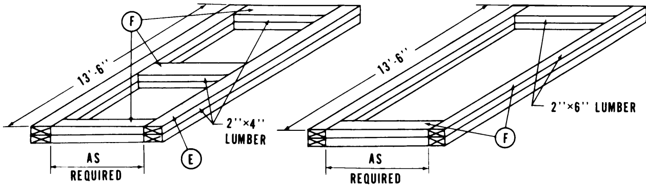
DETAIL 1
