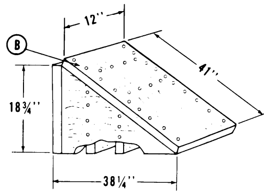
ASSEMBLED VIEW
